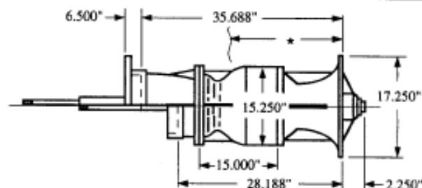
LINESHAFT TURBINE
