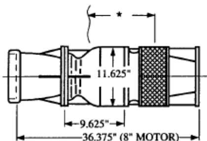
SUBMERSIBLE TURBINE
