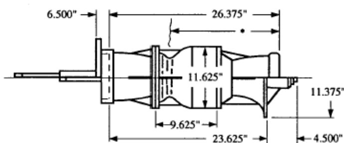
LINESHAFT TURBINE
