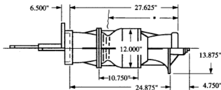
LINESHAFT TURBINE
