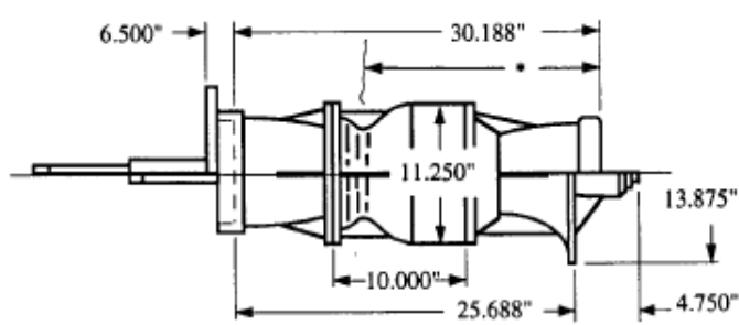
LINESHAFT TURBINE
