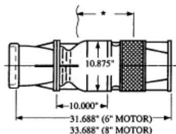
SUBMERSIBLE TURBINE
