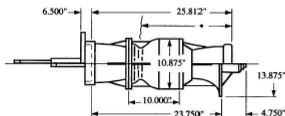
LINESHAFT TURBINE
