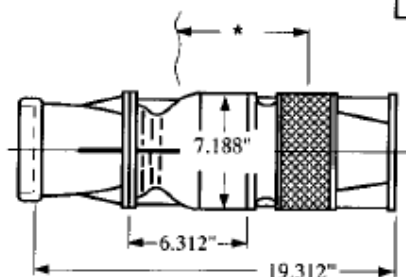
SUBMERSIBLE TURBINE
