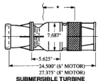
SUBMERSIBLE TURBINE
