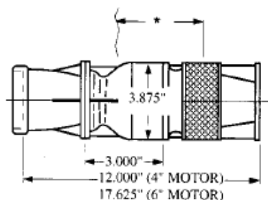
SUBMERSIBLE TURBINE
