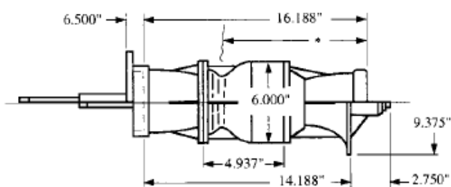
LINESHAFT TURBINE
