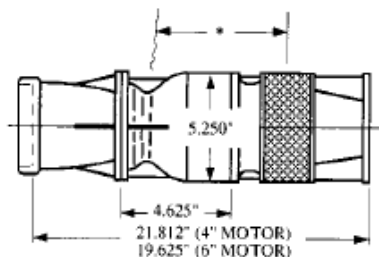
SUBMERSIBLE TURBINE
