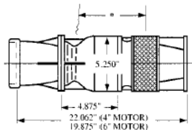
SUBMERSIBLE TURBINE
