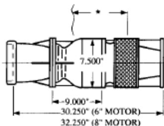
SUBMERSIBLE TURBINE
