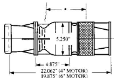
SUBMERSIBLE TURBINE
