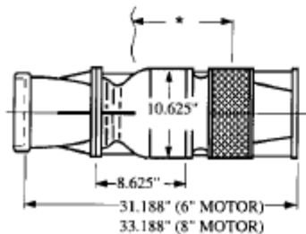
SUBMERSIBLE TURBINE
