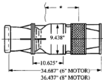
SUBMERSIBLE TURBINE
