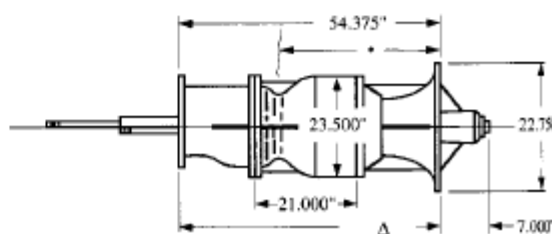
LINESHAFT TURBINE
