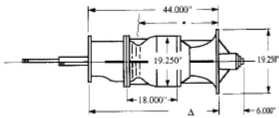
LINESHAFT TURBINE
