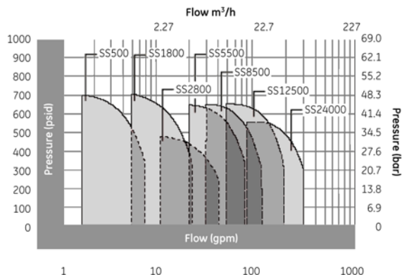
Figure 2: Performance Curve (60Hz) (Logarithmic Scale)
